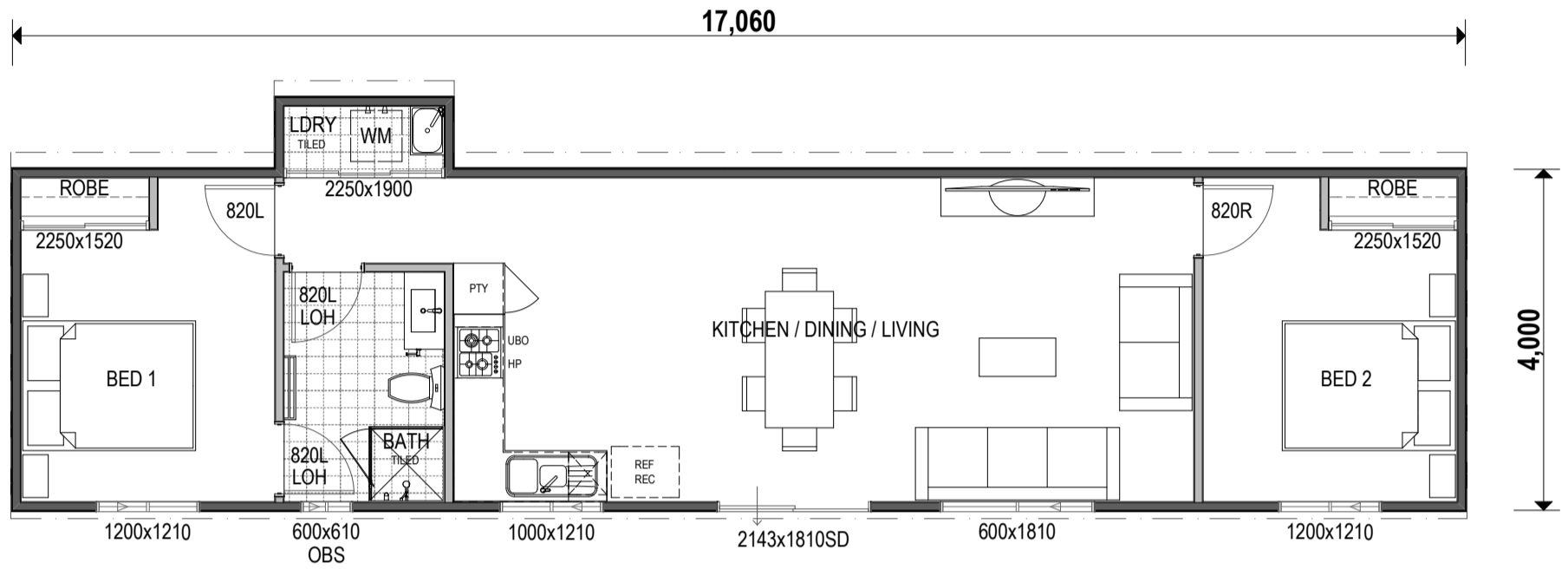
2 x BED - 70m 2
