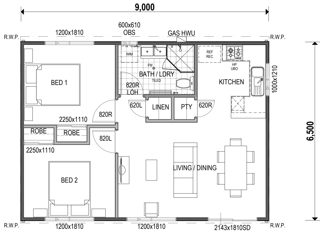
2 x BED - 58.50m 2
