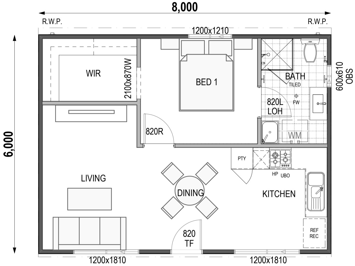
VERSION 2 THE DIANELLA - 1 x BED AS DISPLAYED W/ LDRY - 48m 2
