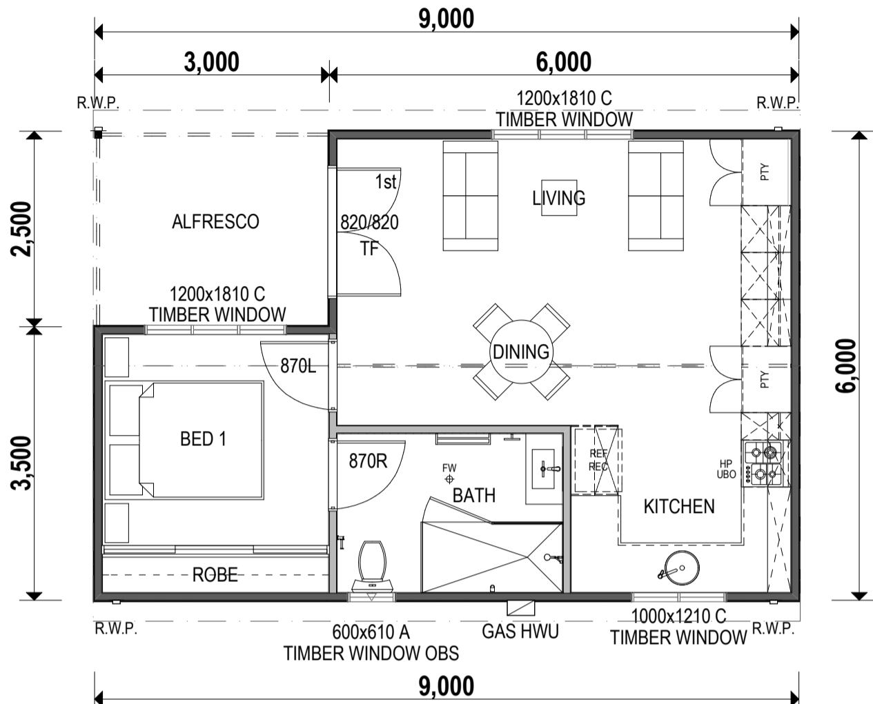
DALKEITH - AS DISPLAYED - 46.50m 2 + ALFRESCO
