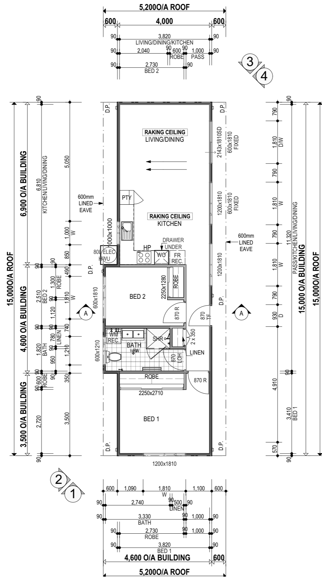
FLOOR PLAN 1:100
