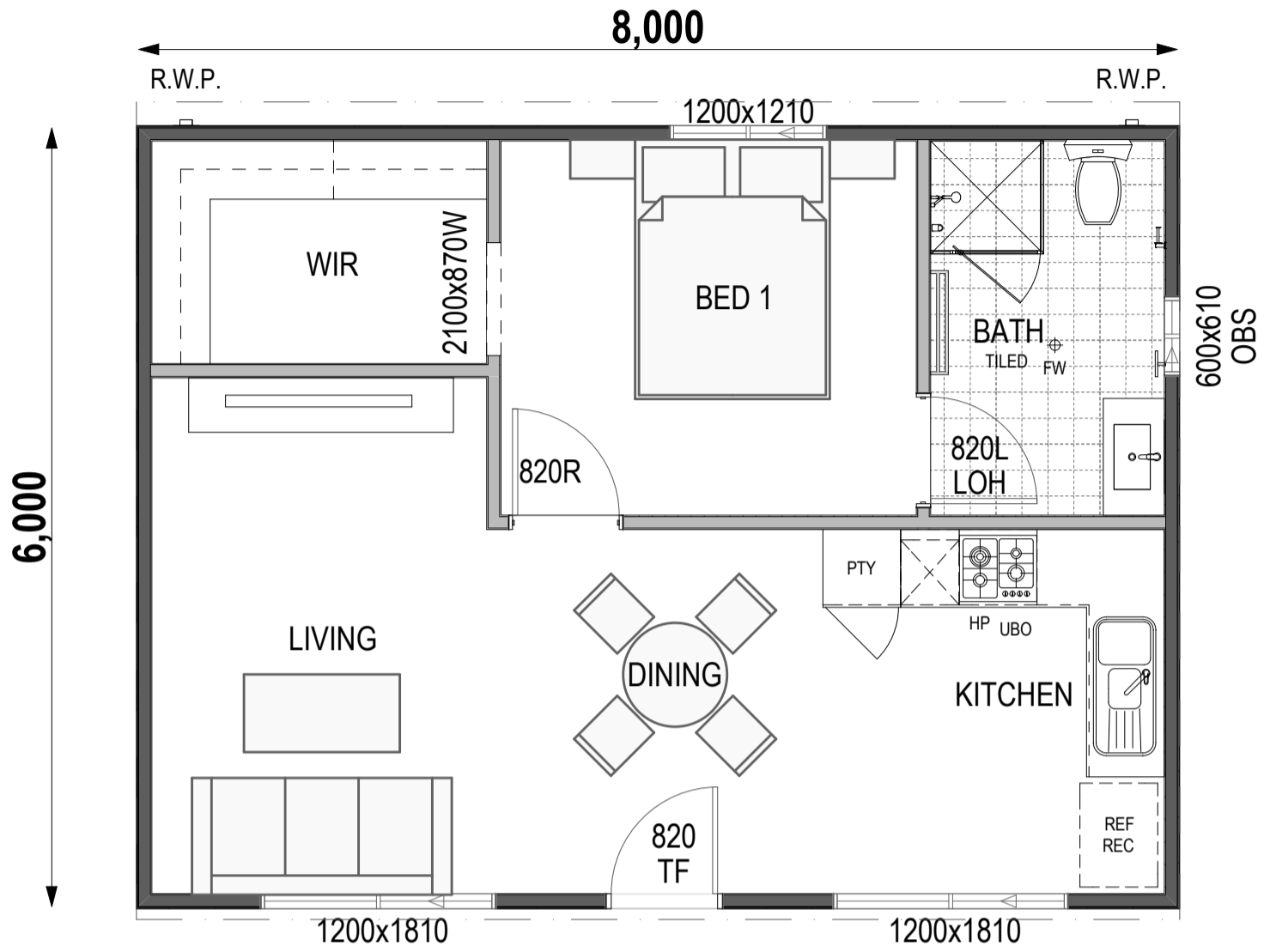
THE DIANELLA - 1 x BED AS DISPLAYED - 48m 2
